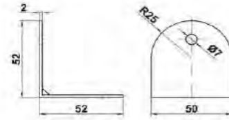
INOX NAUGLICA MODEL 100
